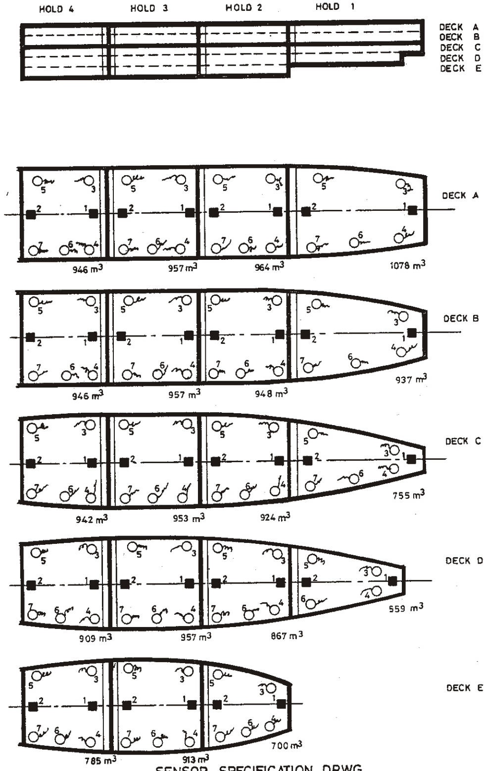
SENSOR SPECIFICATION DRWG.
