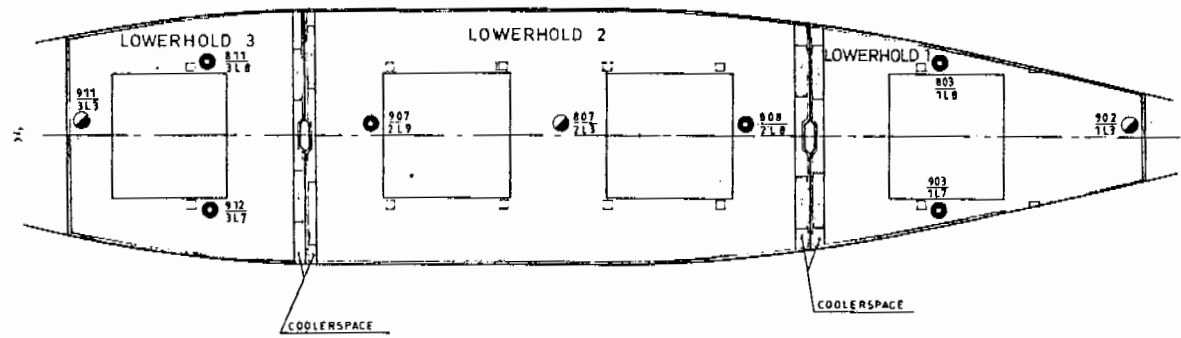
VIEW TANKTOP
