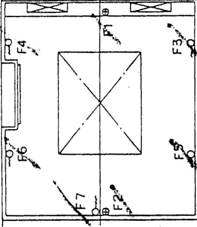
NO. 4 A REF. CARGO HOLD
