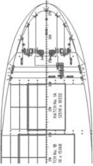
CARGO DECK 1 - 16600
